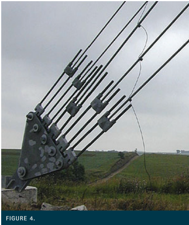
FIGURE 4. Original grounding connection at an outer anchor. High ground resistance and questionable connections enabled lightning to bypass this grounding system, causing damage to the anchor concrete, lower left. Note the zigzag path of the grounding conductor that reduced the system's effectiveness.
